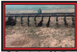
Toolbar w/coulters & fertilizer knives
